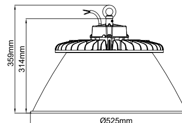
Tall Reflector
