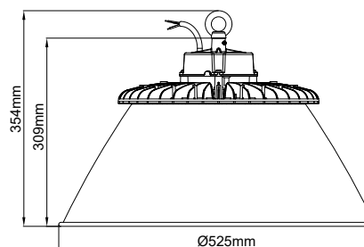
Tall Reflector
