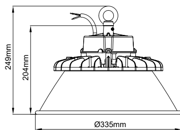
Universal Reflector
