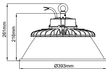
Universal Reflector
